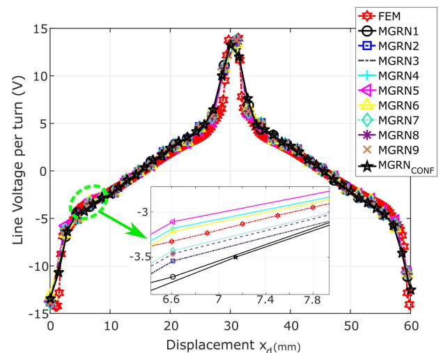
Fig. 15. Line voltage per turn versus displacement.
